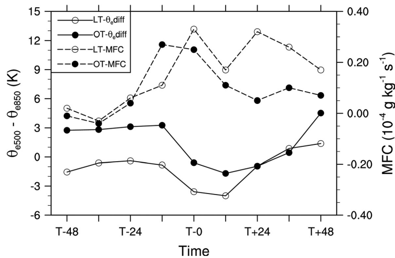
Fig. 11. Time series of the equivalent potential temperature difference between 500 and 850 hPa ( \theta_e diff = \theta_{e500}-\theta_{e850} , solid lines) and CIMFC (dashed lines) for LT (open circle) and OT (blackened circle). These values are the average over grids in the box shown in Fig. 9a.
